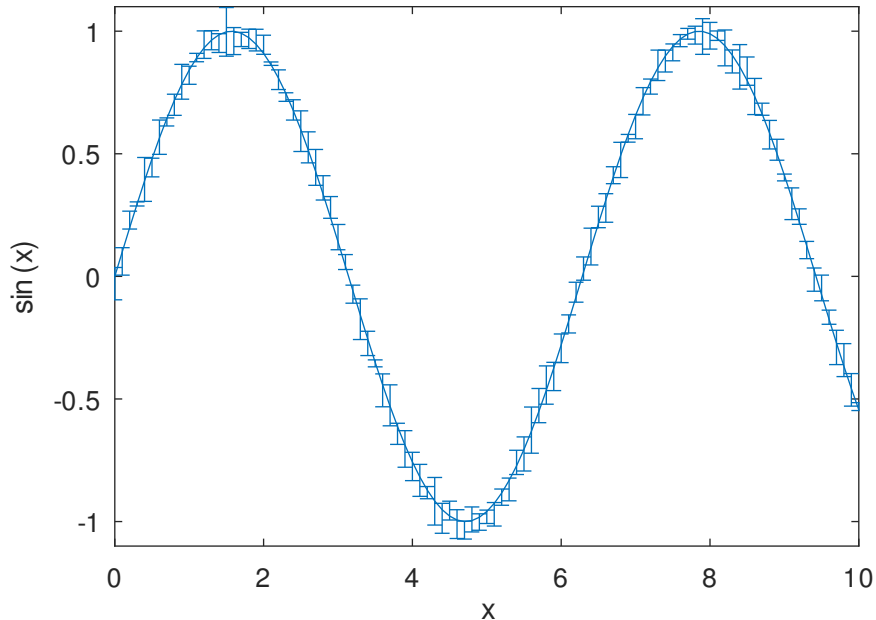
Errorbar plot of \sin(x)
