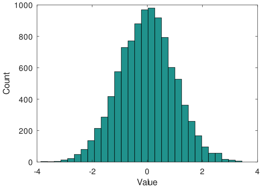
Histogram of 10,000 normally distributed random numbers
