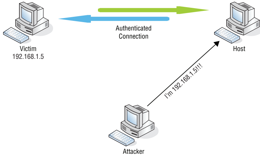
FIGURE 12.4 Spoofing
