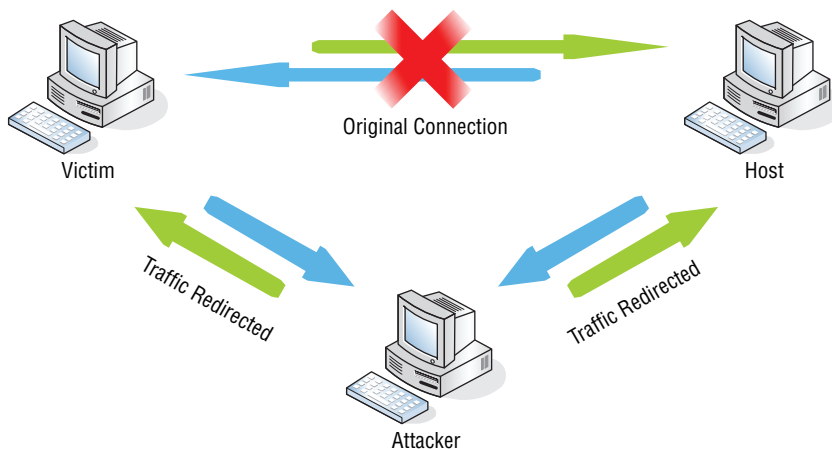
FIGURE 12.8 MITM attack
