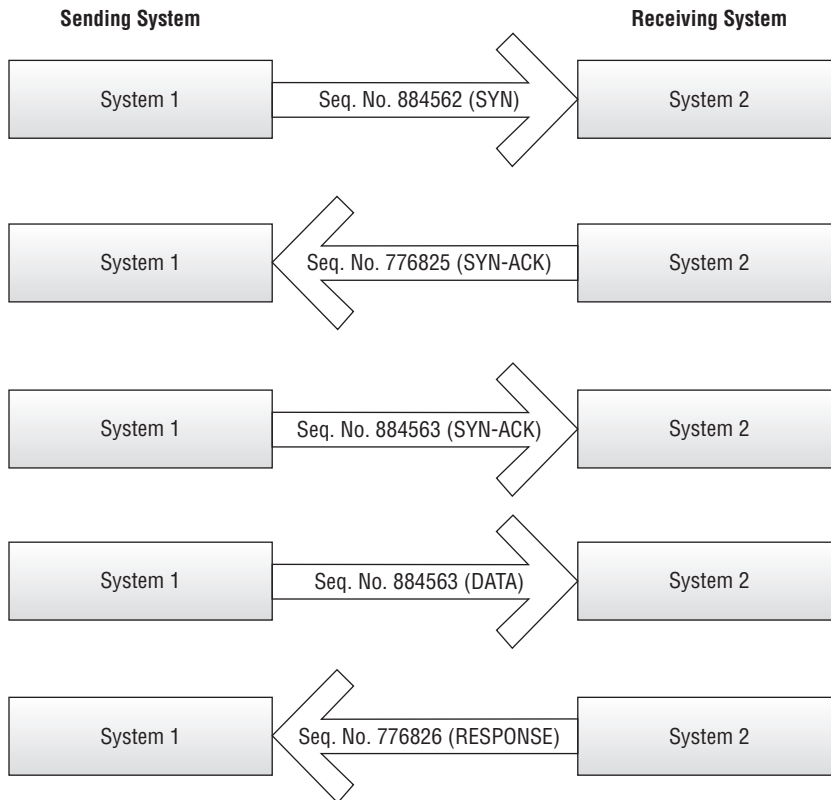
FIGURE 2.8 TCP sequencing
