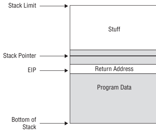
FIGURE 11.1 Basic program stack
