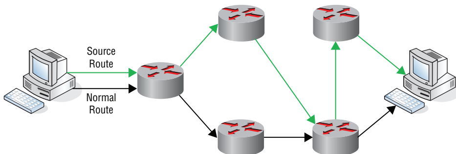
FIGURE 12.5 Source routing
