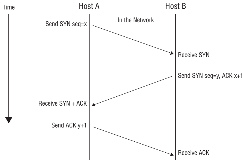
FIGURE 5.1 The three-way handshake
